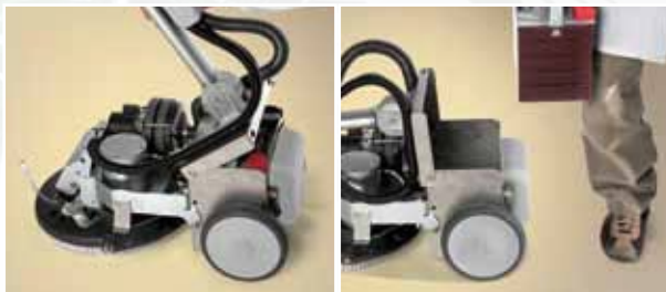
Vispa 35 B The battery compartment is easily accessible for quick battery replacement
